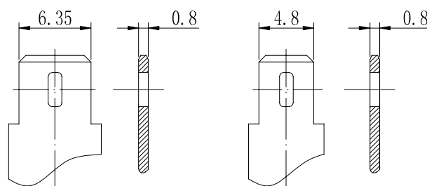
Terminal T2
