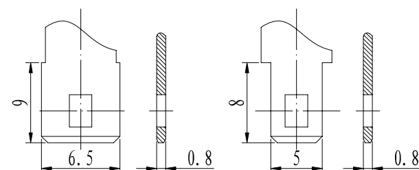
Positive terminal
