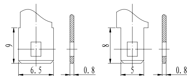
Positive terminal
