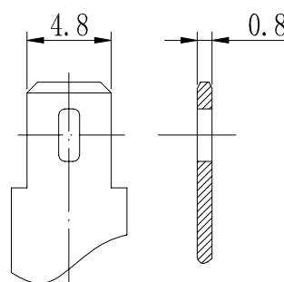
Terminal T1
