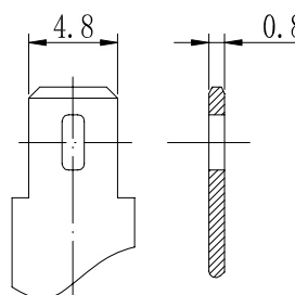
Terminal T1
