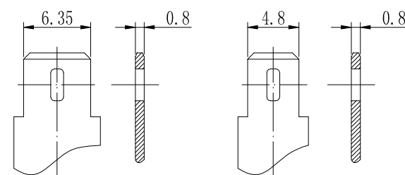
Terminal T2
