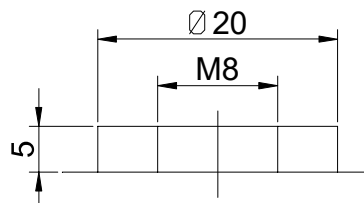
Terminal T10
